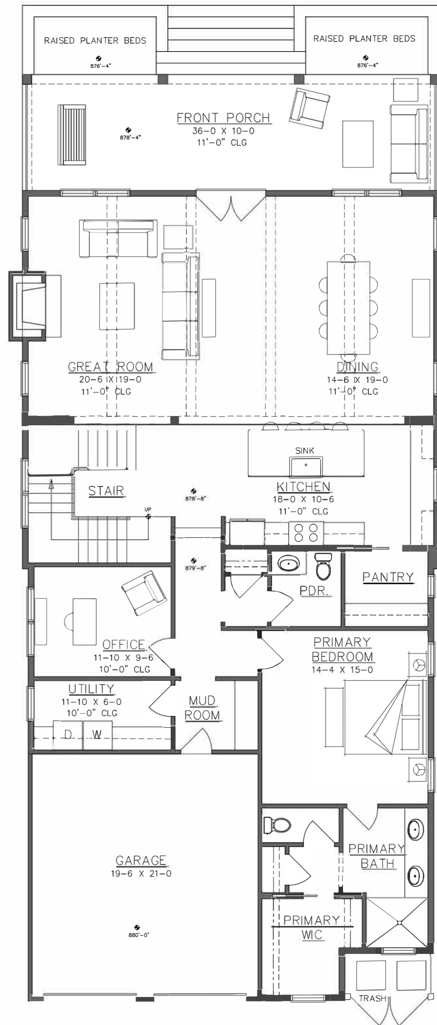
FIRST FLOOR PLAN 2,028 SF
