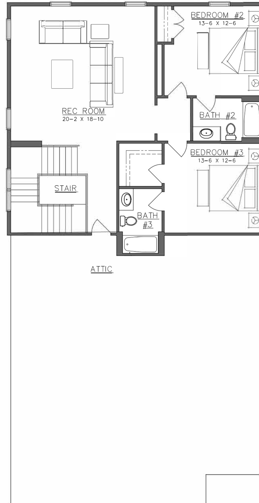
SECOND FLOOR PLAN 1,118 SF
